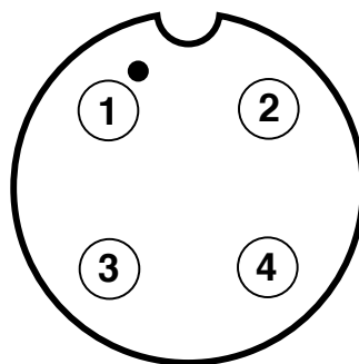
MP406 4-pin female cable entry view
